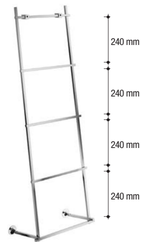
C480 Scaletta 4 barre Ladder with 4 bars L. 346 H. 1080 P. 210 mm
