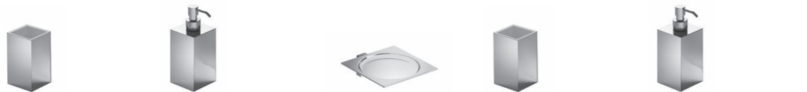
C402 C423 C401 C462 C463 Portaspazzolini a parete Wall-mounted toothbrush holder L. 60 H. 115 P. 70 mm Dosatore sapone liquido a parete Wall-mounted liquid soap dispenser L. 60 H. 157 P. 70 mm Portasapone a parete Wall-mounted soap dish L. 100 H. 38 P. 116 mm Portaspazzolini da appoggio Free-standing toothbrush holder L. 60 H. 115 P. 60 mm Dosatore sapone liquido da appoggio Free-standing liquid soap dispenser L. 60 H. 157 P. 60 mm
